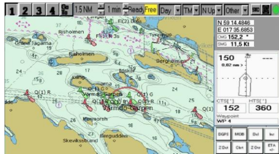
Prototype ECDIS G8 in Classic mode
